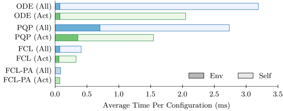
Fig. 3: The timing performance for the ODE, PQP, FCL, and FCL-PA on 259,135 collision checks recorded from the table-clearing task. Each pair of bars shows the effect of checking \square \blacksquare all links and \square \blacksquare only those moved by the active DOFs. Each stacked bar shows the time required for the \blacksquare \square environment and \square \square self-collision check. No such distinction exists for \square \square FCL-PA.
